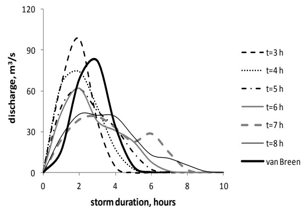
Figure 6. The Hydrographs Generated using Rainfall Intensity Distribution
